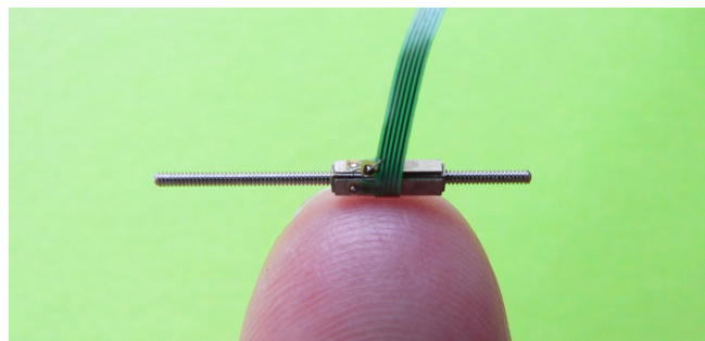
Figure 1: Linear SQUIGGLE motor measures only 1.55 x 1.55 x 6 mm
