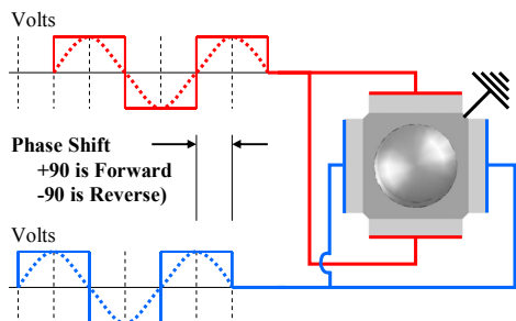
Figure 4: Two-phase motor drive signals (sinusoidal or square wave)
